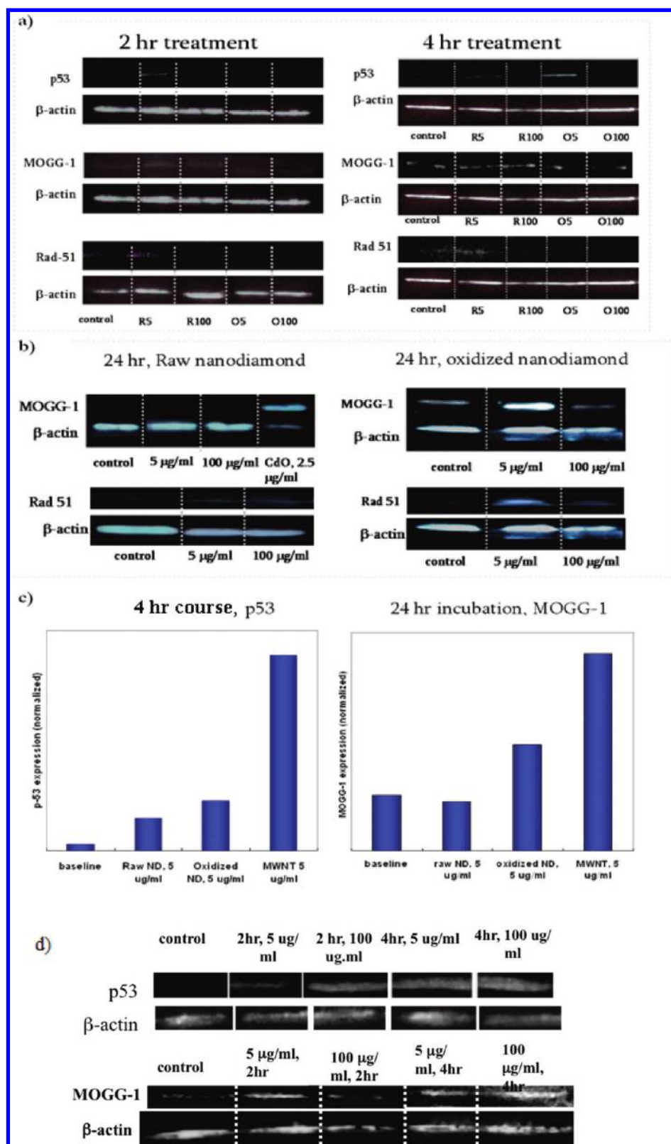
Figure 1. (a) Short-term responses as shown in p53, MOGG-1, and Rad-51. Note that R5, R100, O5, and O100 represent R-NDs at 5 \mu\text{g/mL} , R-NDs at 100 \mu\text{g/mL} , O-NDs at 5 \mu\text{g/mL} , and O-NDs at 100 \mu\text{g/mL} , respectively. (b) Longer term response, 24 h incubation; (c) quantified DNA damage (as in protein expression) compared with MWNTs. (d) Responses in p53 and MOGG-1 from MWNT samples in ES cells.
