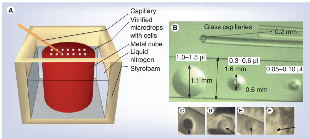
Figure 3. Droplet vitrification. (A) The solid surface vitrification device. A metal cube covered with aluminum foil was partially submerged into liquid nitrogen. Microdroplets of vitrification solution containing the oocytes were dropped onto the cold upper surface of the metal cube and are instantaneously vitrified. (B) The modified minimum drop size technique. Droplets of various sizes were placed on glass cover slips using capillaries. (C–F) Droplets generated by MDS technique during vitrification with (C) ice crystals, (D & E) with fractures, and (F) without crystallization and fractures using CPA concentration reduced by 50% of those used in (C). Reproduced with permission from [54] © (2010) Elsevier.
