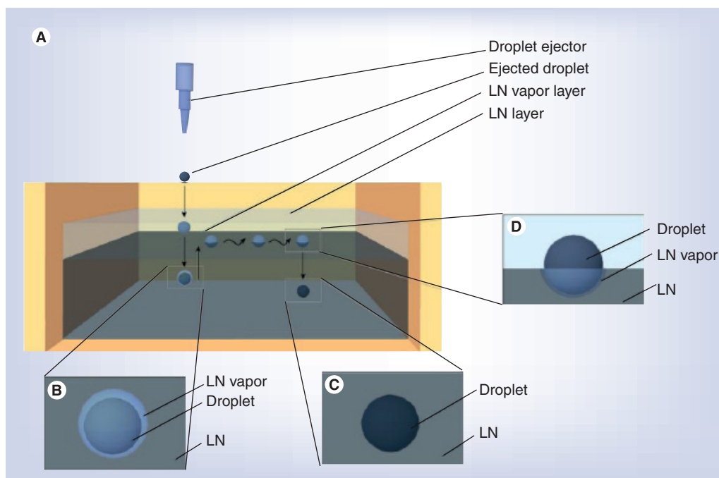
Figure 2. Generation of droplets and levitation of droplets on top of liquid nitrogen.
