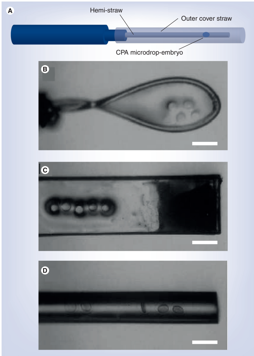
Figure 1. Minimum volume vitrification carriers. (A) Hemi-straw, which was inserted into a 0.5 ml straw for storage, (B) Cryoloop [48], (C) Cryotop [48] and (D) gel loading tip [48]. Scale bar = 400 \mu\text{m} . (B–D) Reproduced with permission from [48] © (2011) Elsevier.
