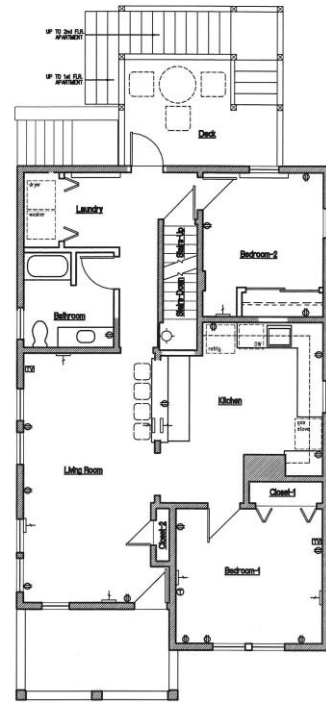
CWRU 1144 Fairfield Avenue Scheme A - New Floor Plan 11/7/11 1/2" = 1'-0" 0 2' 4' 10' 1' 3' 5'
