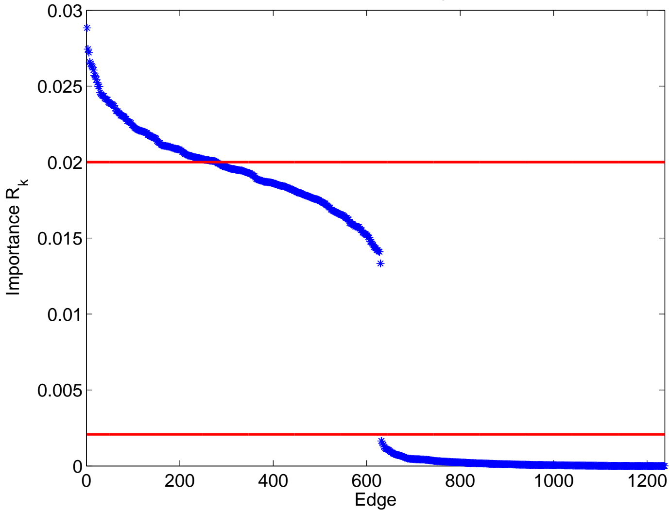
Erdos–Renyi on 50 nodes: Edge Importance
